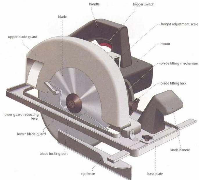
CIRCULAR SAW
