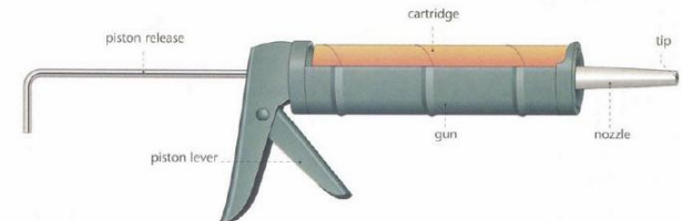
CAULKING GUN
